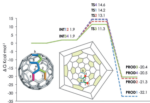
Figure 3. Gibbs energy profile calculated at the BP86-D/TZP//BP86-D/DZP level of theory for the BH cycloaddition to selected non-equivalent bonds of Sc_3N@D_{3h}-C_{80} (in kcal mol -1 ) and the representation of the five non-equivalent [6,6] bonds: pyrene bond type bond 1; pyracylene bond 5; type B bonds 2, 3, 4, and 5; and four [5,6] type D corannulene bonds a–d.
